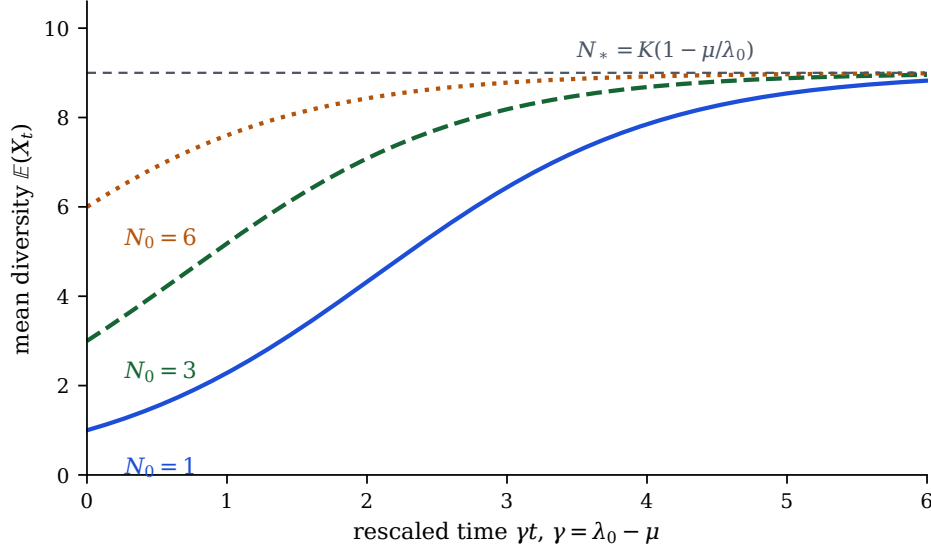
Figure 1.7: Mean diversity (1.38) of the logistic speciation surrogate for founding diversities N_0 = 1, 3, 6 , with \mu/\lambda_0 = 0.1 and K = 10 , so that N_* = 9 ; the abscissa is the rescaled time \gamma t . Every founding diversity relaxes monotonically to N_* , and the mean of the surrogate coincides with the deterministic solution (1.35) exactly, because the surrogate is linear and its mean therefore closes. The smallest cohort spends a long early interval in near-exponential growth before the diversity dependence binds — and it is over precisely that interval that the surrogate is least trustworthy, since it is there that a single realisation is least like its mean.
