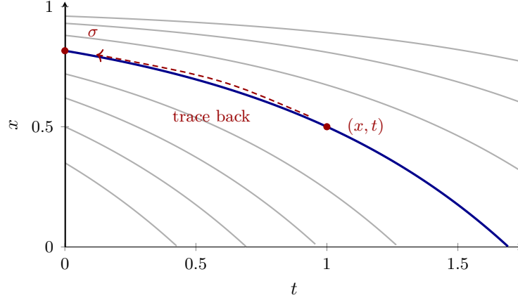
Figure 1.14: Characteristics of the x -equation (1.87), dx/d\tau = \mu(1-x) with \tau = -t , drawn for \mu = 1 . Each grey curve is one characteristic, x(t) = 1 - (1 - \sigma)e^{\mu t} , labelled by the point \sigma at which it meets the initial surface t = 0 , drawn as the heavy vertical line; together they foliate the domain, and exactly one passes through any given (x, t) . Since G is constant along characteristics, its value at a point is its value at the foot of that point's curve — so solving the equation amounts to running the curve backwards from (x, t) to t = 0 and reading off \sigma , here \sigma = 1 - (1 - x)e^{-\mu t} . The full problem is three-variate; this is its projection onto the (x, t) plane, which is where the cascade starts, because (1.87) does not involve y .
