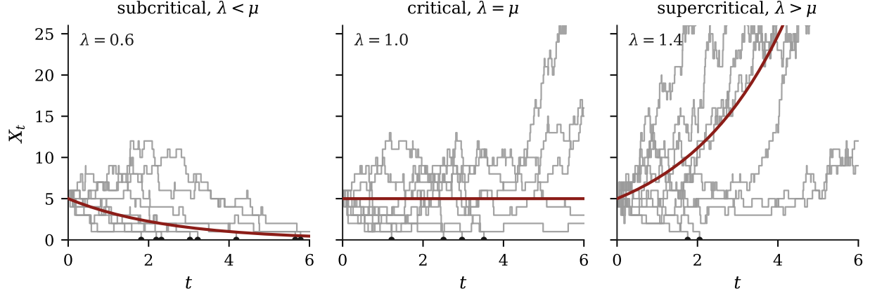
Figure 1.5: Nine realisations of the linear birth–death process (1.22) from X_0 = 5 , with \mu = 1 throughout and the mean Ne^{(\lambda-\mu)t} of (1.61) in red; dots on the axis mark trajectories that reached the absorbing state. The middle panel is the one to dwell on. At criticality the mean is exactly constant, and yet several realisations are already extinct while others have grown fourfold — the mean is the same number in both cases, and describes neither. Note also that extinction is not confined to the subcritical panel: a supercritical process still dies out with probability (\mu/\lambda)^N , visible here as the paths that fail early on the right.
